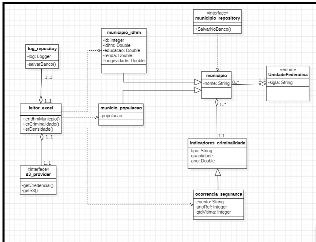
Figura 36 – Diagrama de classes da Safety Intelligence.
